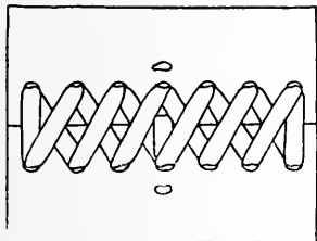
FIG. 225. STRAIGHT STITCH BELT LACE—FLESH SIDE.
